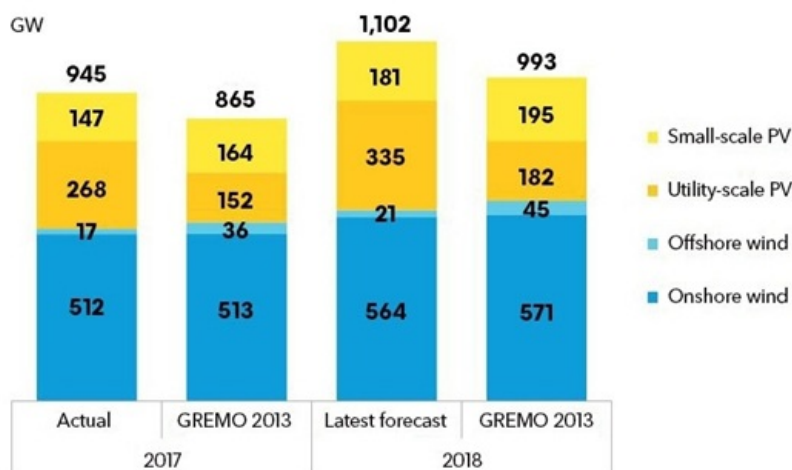
Global installed wind and solar in 2017 and 2018: Comparison of 2013 forecasts versus today
