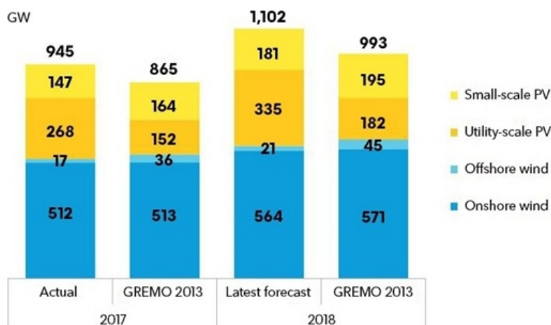
Global installed wind and solar in 2017 and 2018: Comparison of 2013 forecasts versus today
